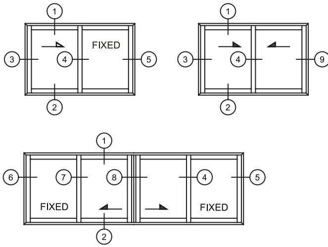
TYPICAL ELEVATION
