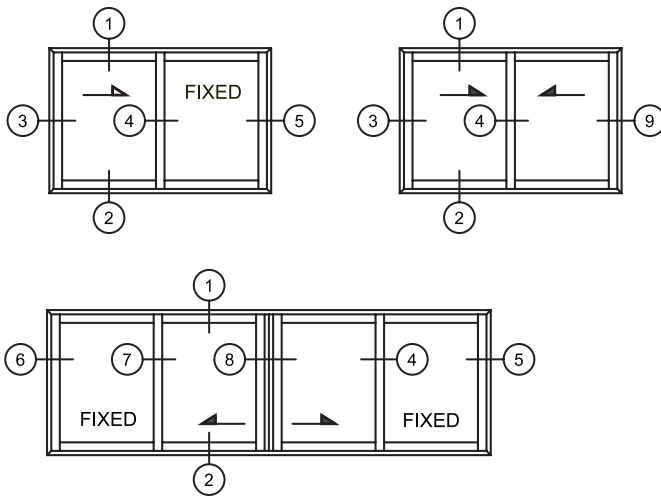
TYPICAL ELEVATION
