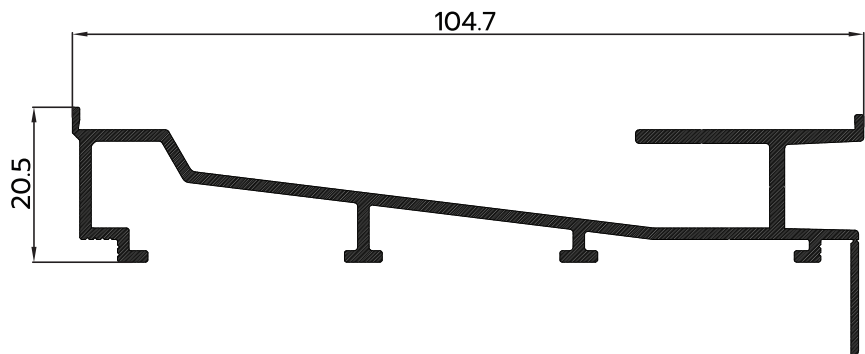
P-003399 Subsills
