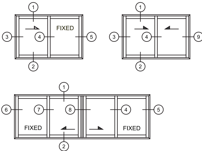
TYPICAL ELEVATION
